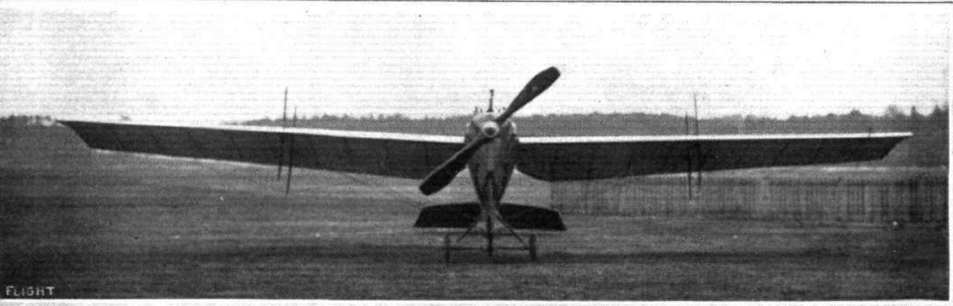
THE MARTIN HANDASYDE, as seen from different points around the machine.
