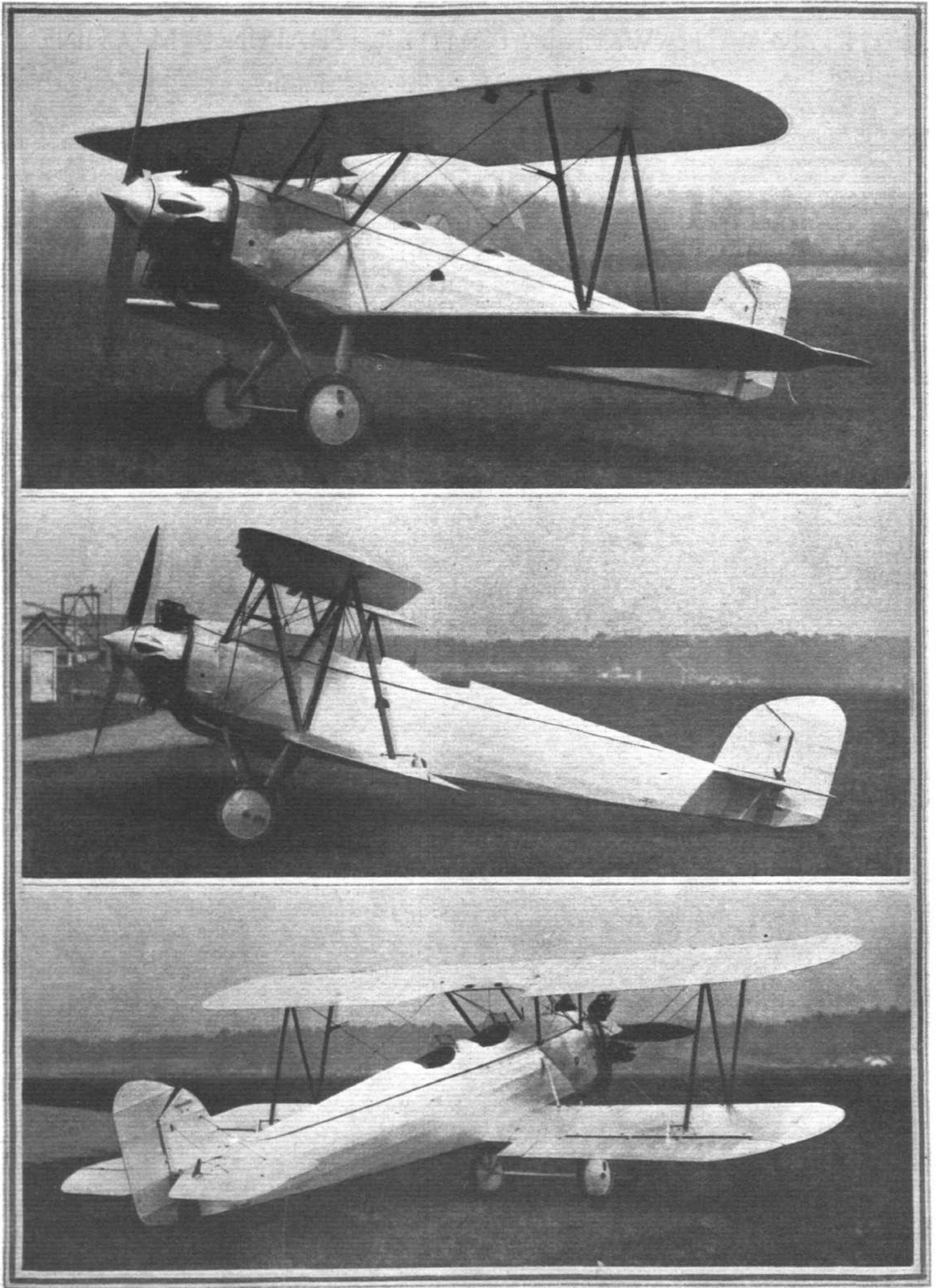
A NEW TRAINING MACHINE: Three views of the Hawker "Tomtit" all-metal biplane. Note the pronounced stagger and slightly backswept wings. The engine is an Armstrong-Siddeley "Mongoose" ["FLIGHT" Photographs
