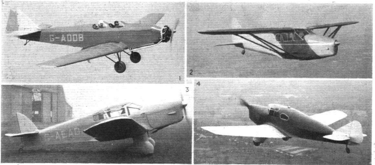
OUTSTANDING CIVIL TYPES : Four machines which made their first appearance during 1935 : (1) the B.A. Swallow with Pobjoy 80 h.p. Cataract engine ; (2) the Heston Phoenix five-seater with 200 h.p. Gipsy Six ; (3) the Percival Vega Gull four-seater with Gipsy Six ; (4) the Miles Merlin five-seater with Gipsy Six. ( Flight photographs.)
