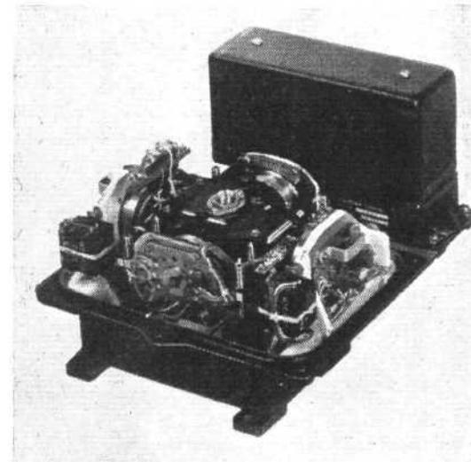
Sperry V.L.G.2 precision vertical gyro
