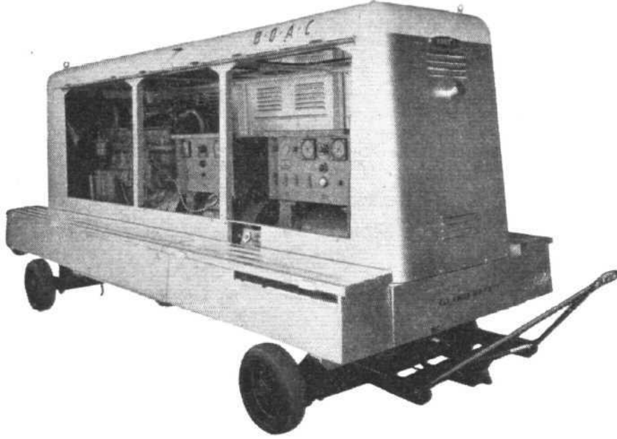
Murex ground power unit, as recently supplied to BOAC, capable of supplying 2,000A for engine starting
