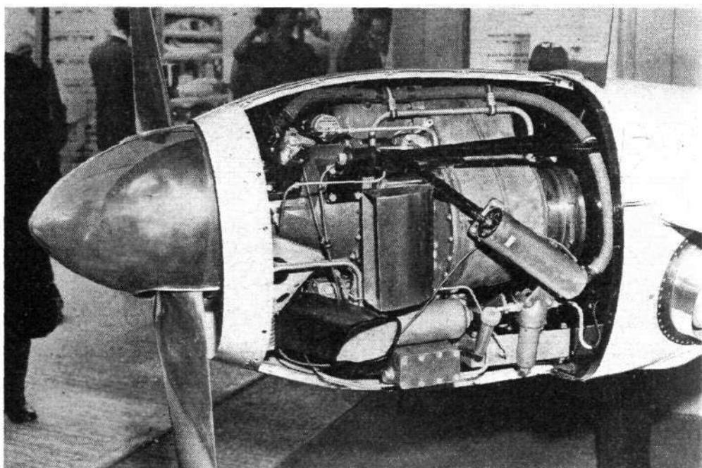
Rover T.P.90 turboprop
