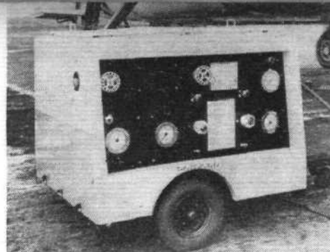
Low-pressure version of the Dunlop mobile air-bottle engine starter trolley in service with Irish International Boeings
