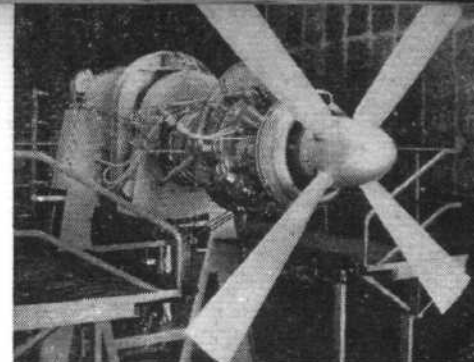
Rolls-Royce Dart torque-measuring bulkhead for a Braathens test house, constructed by John Curran
