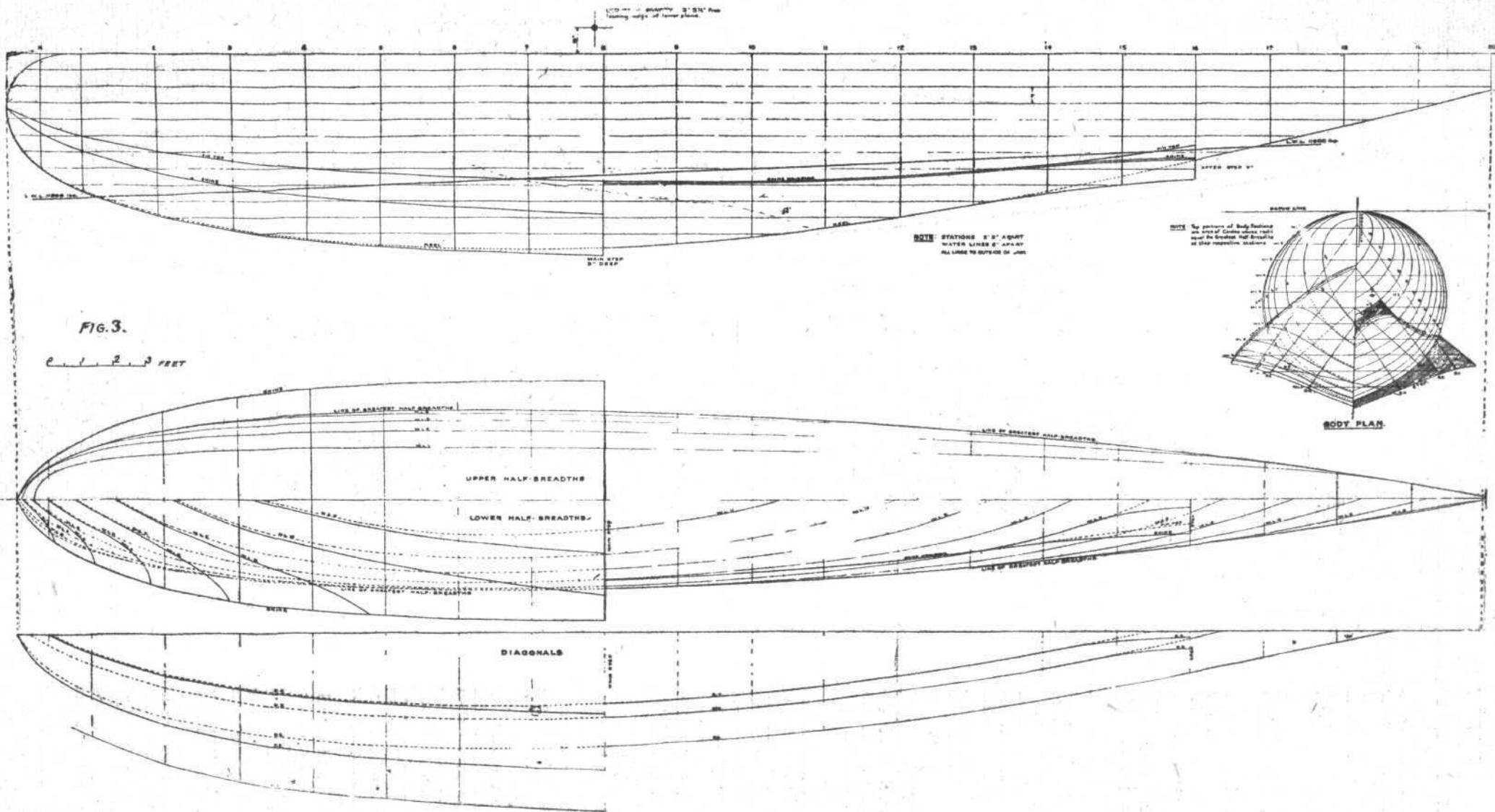
NOTES ON FLYING BOAT HULLS: Fig. 3.—The lines of " P.5 " (Phœnix Cork). Note.—The stations are 2 ft, 3 ins. apart, and the water lines 6 ins. apart ; all lines to outside of skin. The top portions of the body sections are arcs of circles, whose radii equal the greatest half-breadths at their respective stations. (See pages 546 et seq.)
