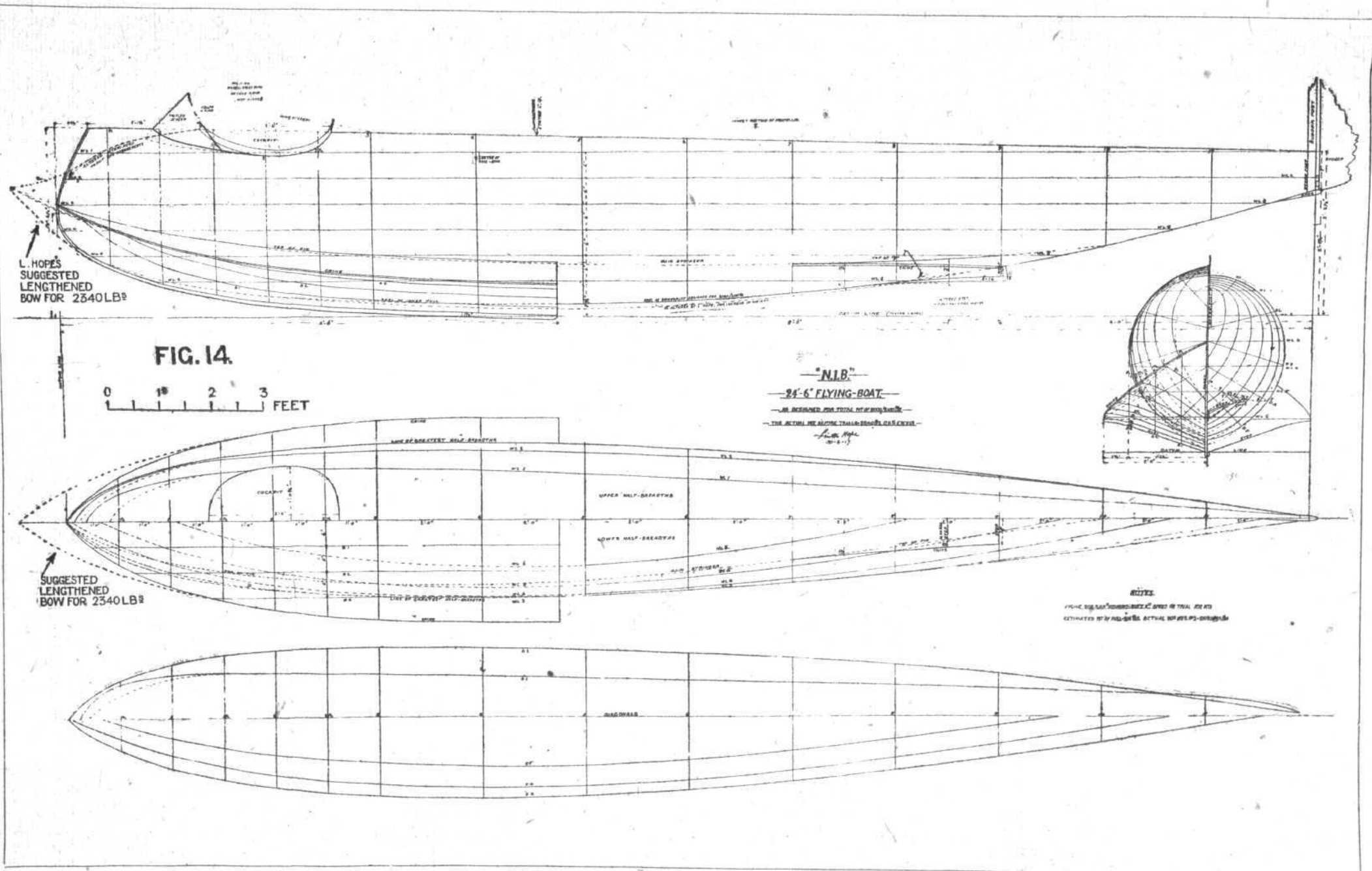
Fig. 14.—Lines of N. 1B, 24 ft. 6 ins. flying boat, as designed for total weight of 2,000–2,100 lbs. The actual weight before trials was 2,340 lbs., an excess of 11½ per cent.
