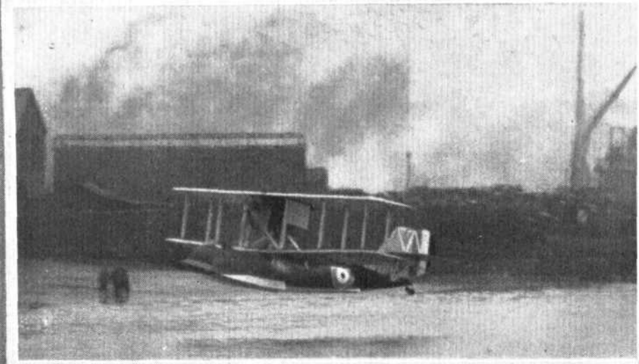
“SEAGULLS” FOR AUSTRALIA: These four views show the Supermarine “Seagull,” piloted by Captain Biard and carrying as passengers Sir Joseph Cook and Squadron-Leader Brown, taking off, in flight, alighting, and moored to a buoy. Two of these photographs give an indication of the poor visibility obtaining at the time of the flight.
