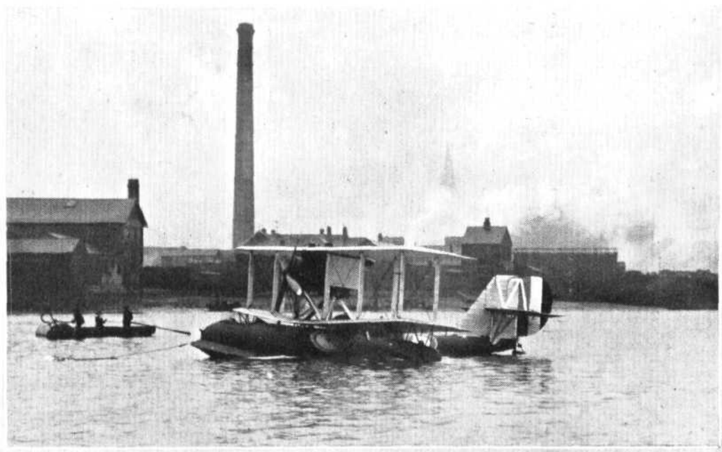
“SEAGULLS” FOR AUSTRALIA: These four views show the Supermarine “Seagull,” piloted by Captain Biard and carrying as passengers Sir Joseph Cook and Squadron-Leader Brown, taking off, in flight, alighting, and moored to a buoy. Two of these photographs give an indication of the poor visibility obtaining at the time of the flight.
