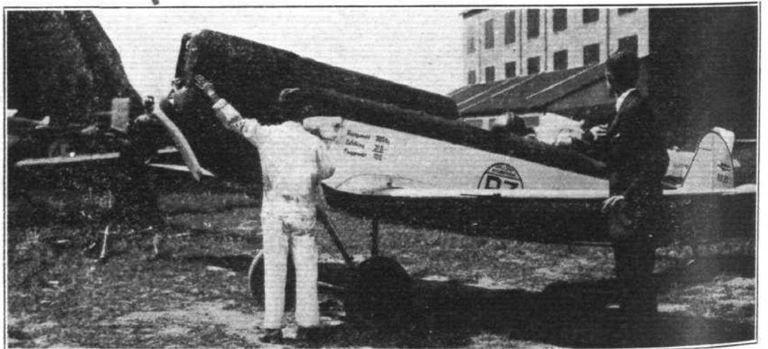
The latest Caudron type 193 low-wing monoplane (85 h.p. Renault). ("FLIGHT" Photo.)
