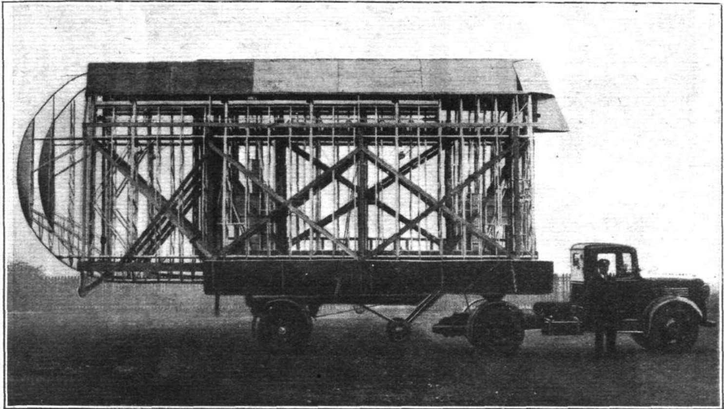
The illustration shows the upper span of a set of BOULTON PAUL Stainless Steel wings for Saro "London" flying boat, ready for the road.
