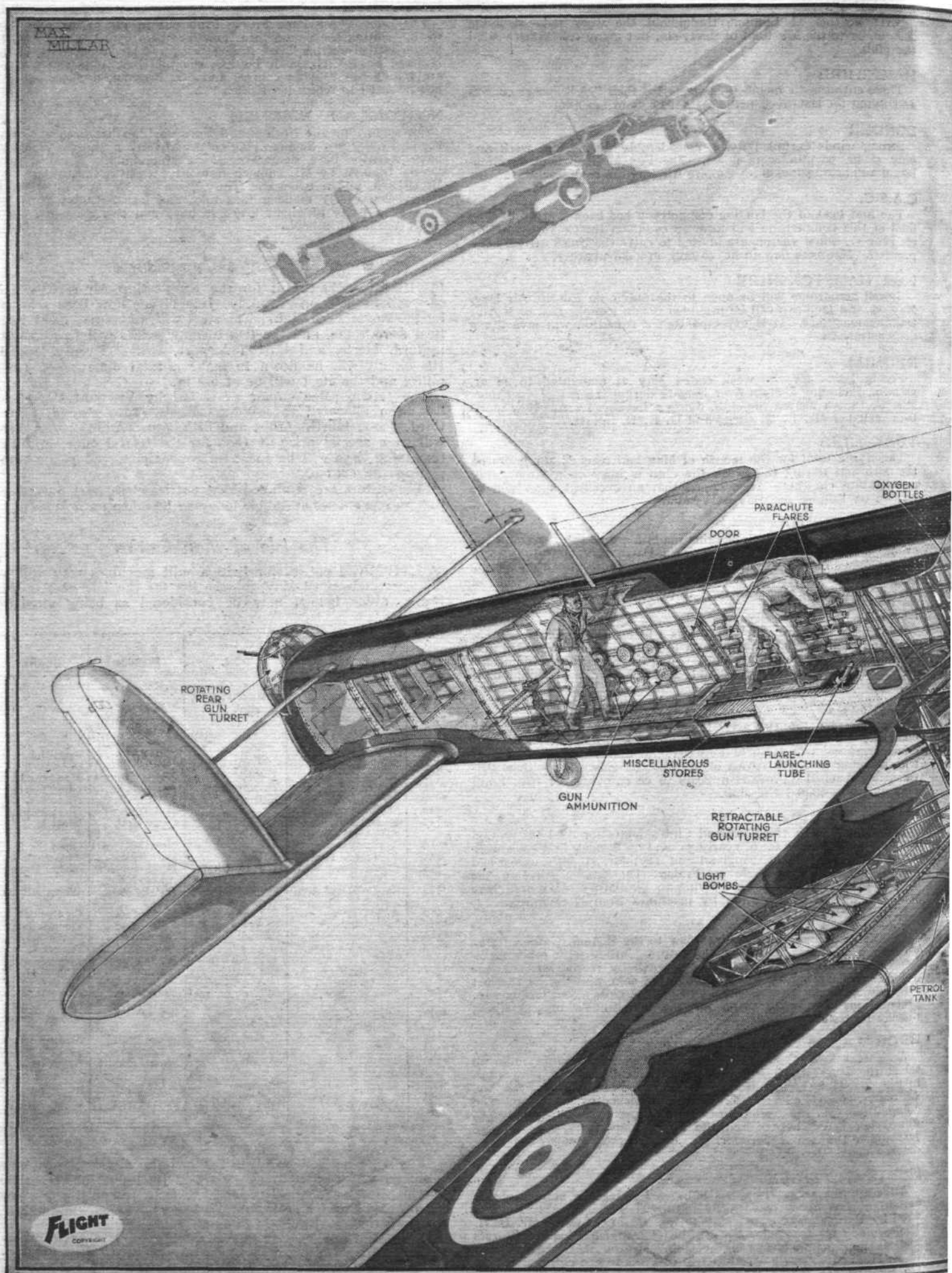
A specially prepared Flight drawing of the Tiger-engined Whitley bomber, a type used by several squadrons of the Royal Air Force. The hand corner shows the nose of the latest type of Whitley—the Mark IV—ordered for service with Rolls-Royce
