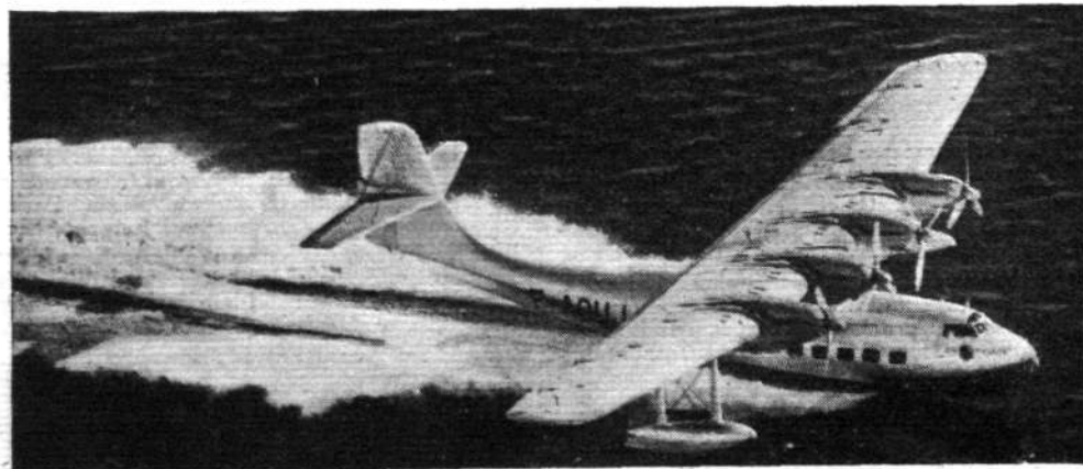
One of Air France's latest types—the Lioré 246—26-passenger flying-boat. Six of these machines have been ordered for the company's Mediterranean services.
