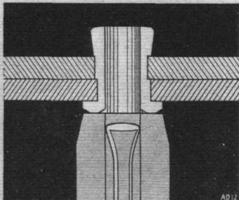
Fig.2. RIVET EXPANDED AND TIGHT
