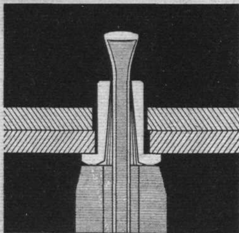
Fig.1. RIVET PLACED & READY FOR EXPANDING
