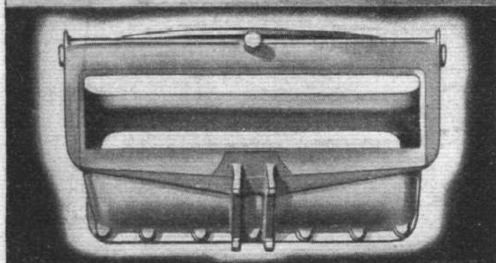
Typical of the sound workmanship that goes into the Fairley Firefly—as supplied to the Royal Navy—are the Class 1 and 2 aluminium castings in DTD 133C alloy by MAYBREY'S.
