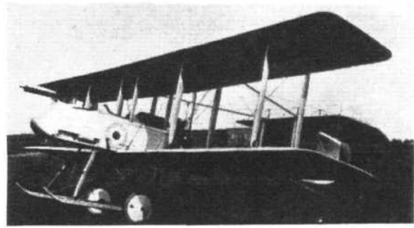
F.B.5 (Gnome) with modified nacelle 1914
