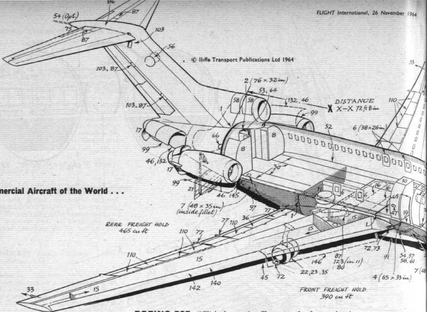
BOEING 727 "Flight International" operators' reference drawing (see page 903 for key; text, page 905)
