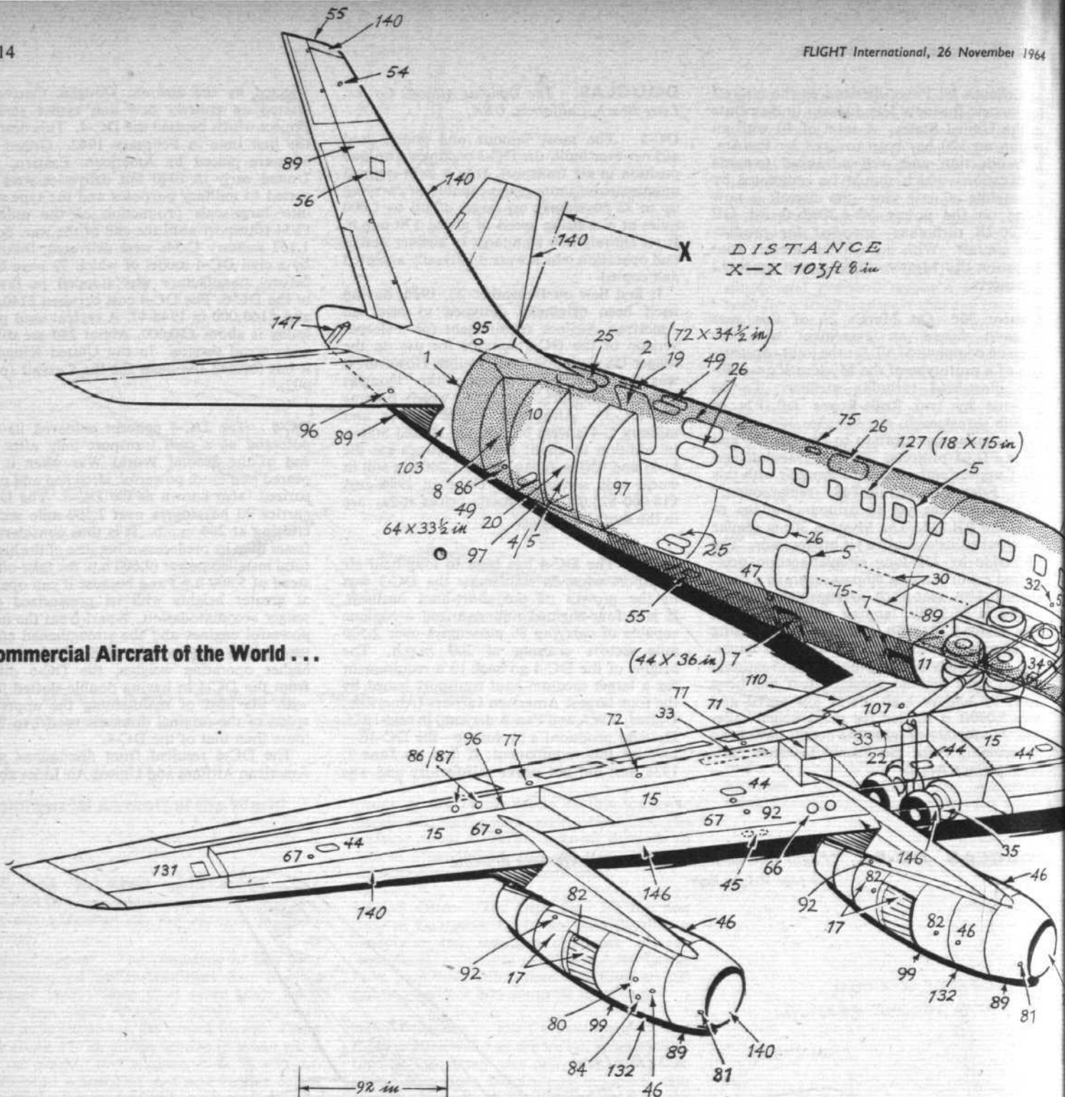
DOUGLAS DC-8F "Flight International" operators' reference drawing (see page 903 for key; text, page 916)
