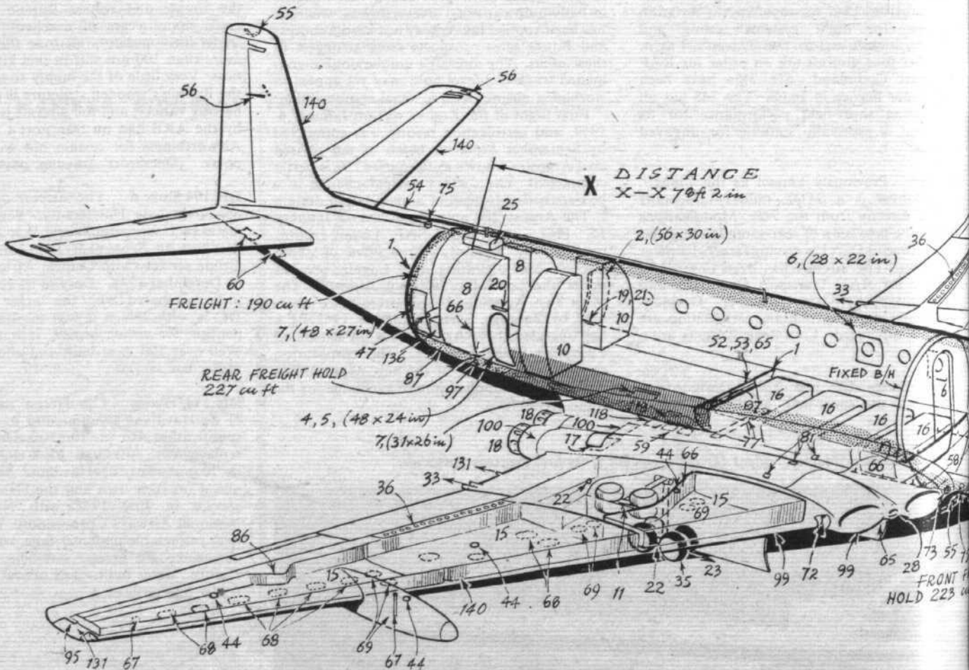
HAWKER SIDDELEY COMET 4C "Flight International" operators' reference drawing (see page 903 for key)
