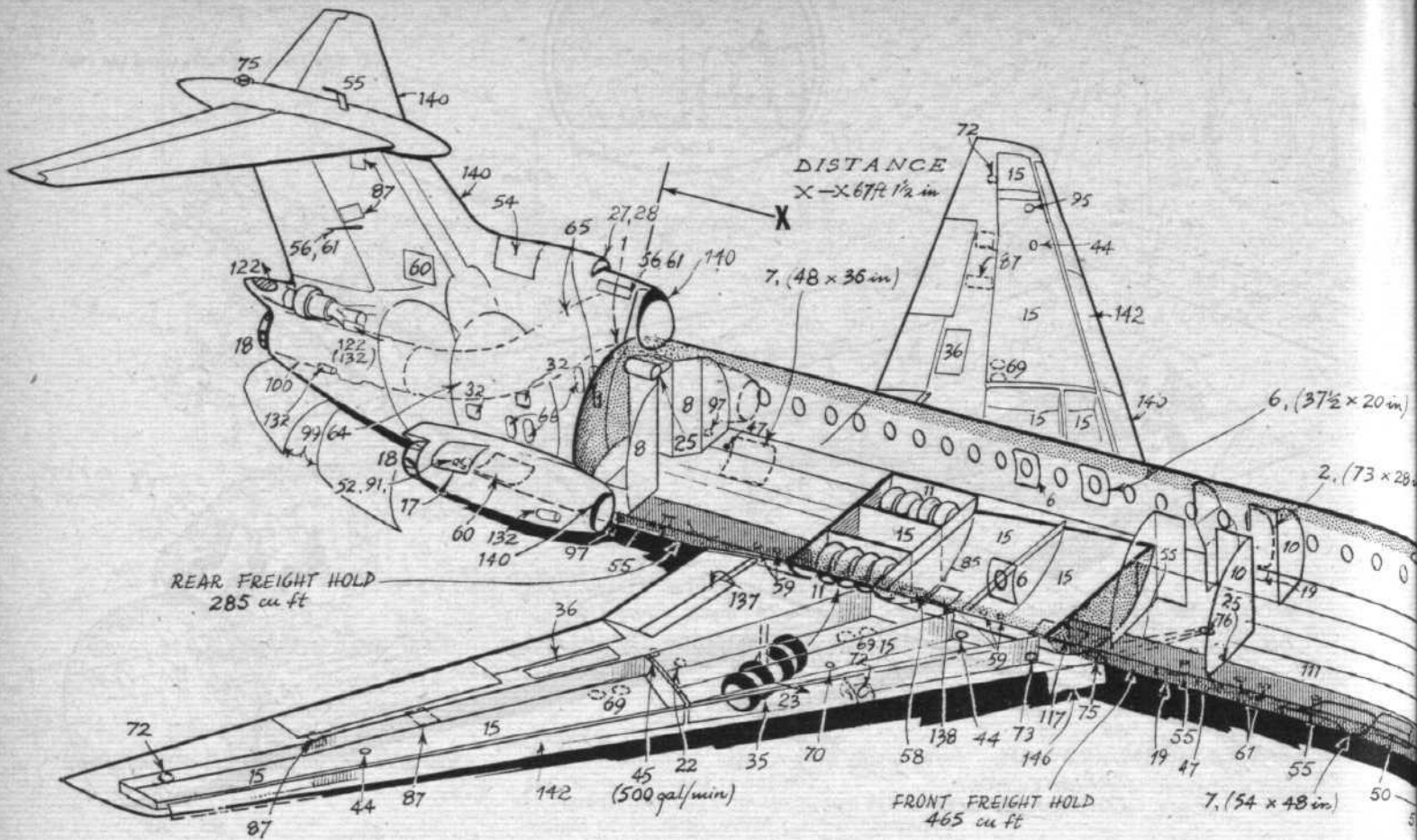
HAWKER SIDDELEY TRIDENT 1E "Flight International" operators' reference drawing (see page 903 for key)
