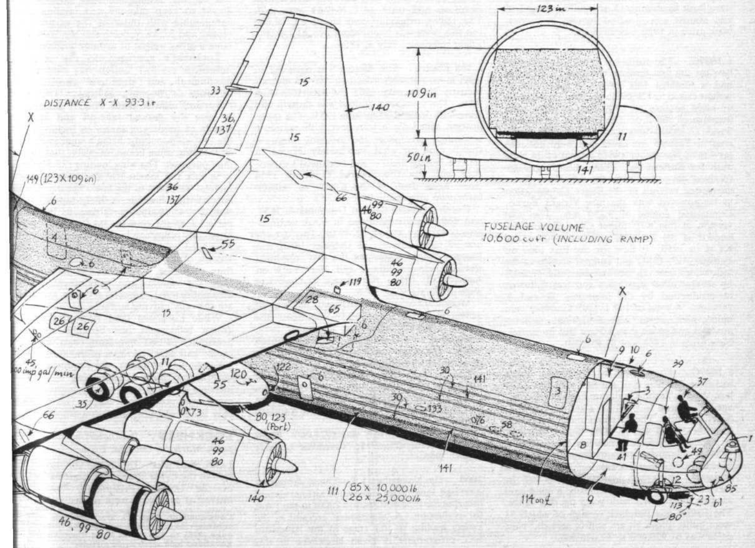
LOCKHEED 301 "Flight International" operators' reference drawing (see page 903 for key; text, page 924)
