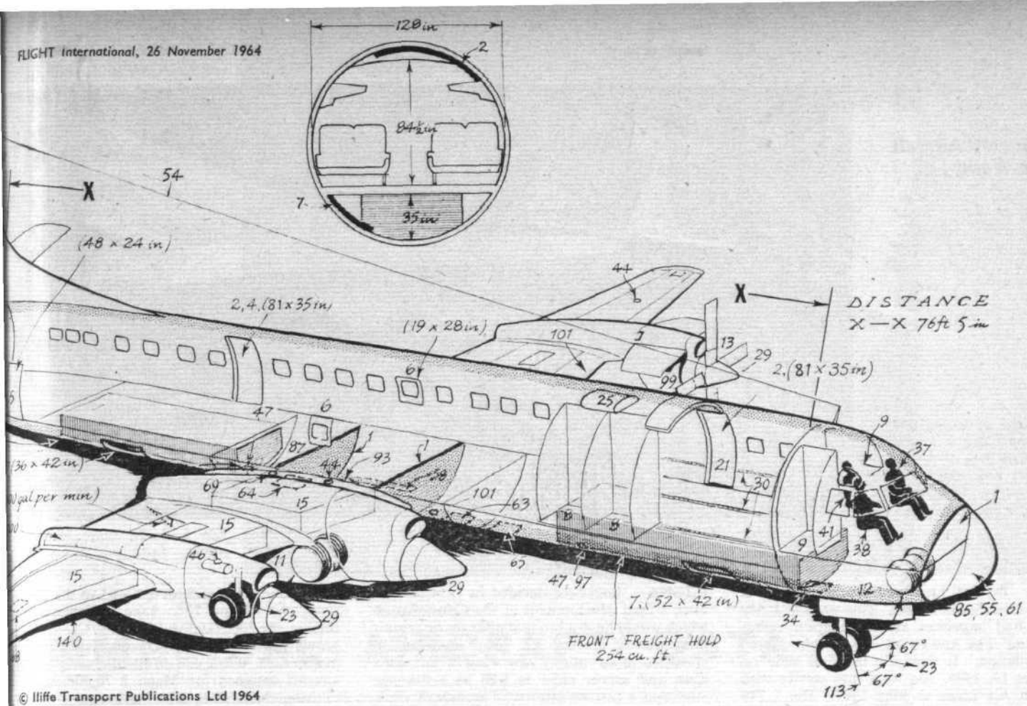
LOCKHEED L.188 ELECTRA "Flight International" operators' reference drawing (see page 903 for key; text, page 924)
